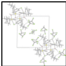
Fig. 2. View of the I structure with the hydrogen bonding along the a axis.
