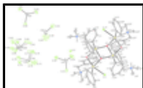
Fig. 1. View of the title compound with the displacement ellipsoids shown on 50% probability level. Most H atoms are omitted for clarity, H atoms involved in hydrogen bonding are shown. Symmetry code: (a) ?x + 2, ?y + 2, ?z .
